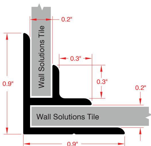
Cross-Section
