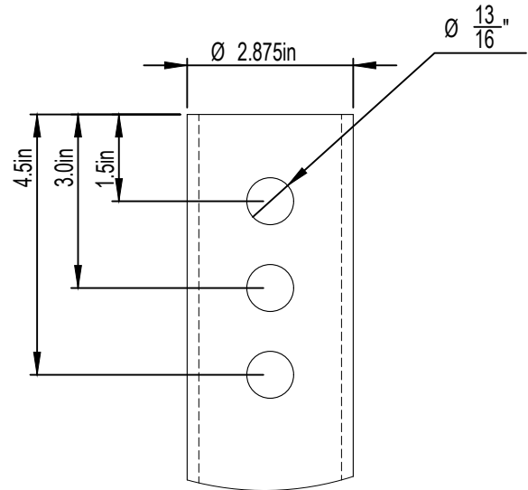
A DETAIL A 1:3
