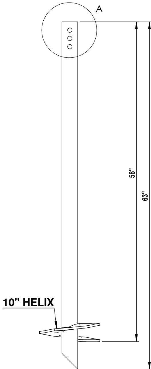
1 2.5" SCH40 SINGLE HELIX 1:10
