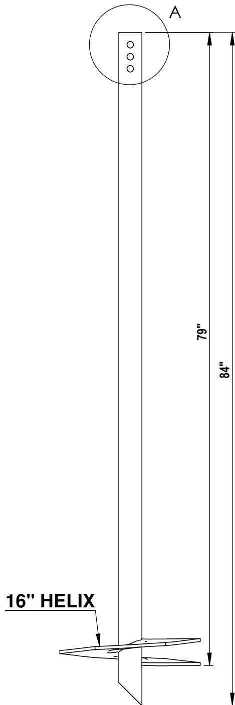
1 2.5" SCH40 SINGLE HELIX 1" = 1' 0"
