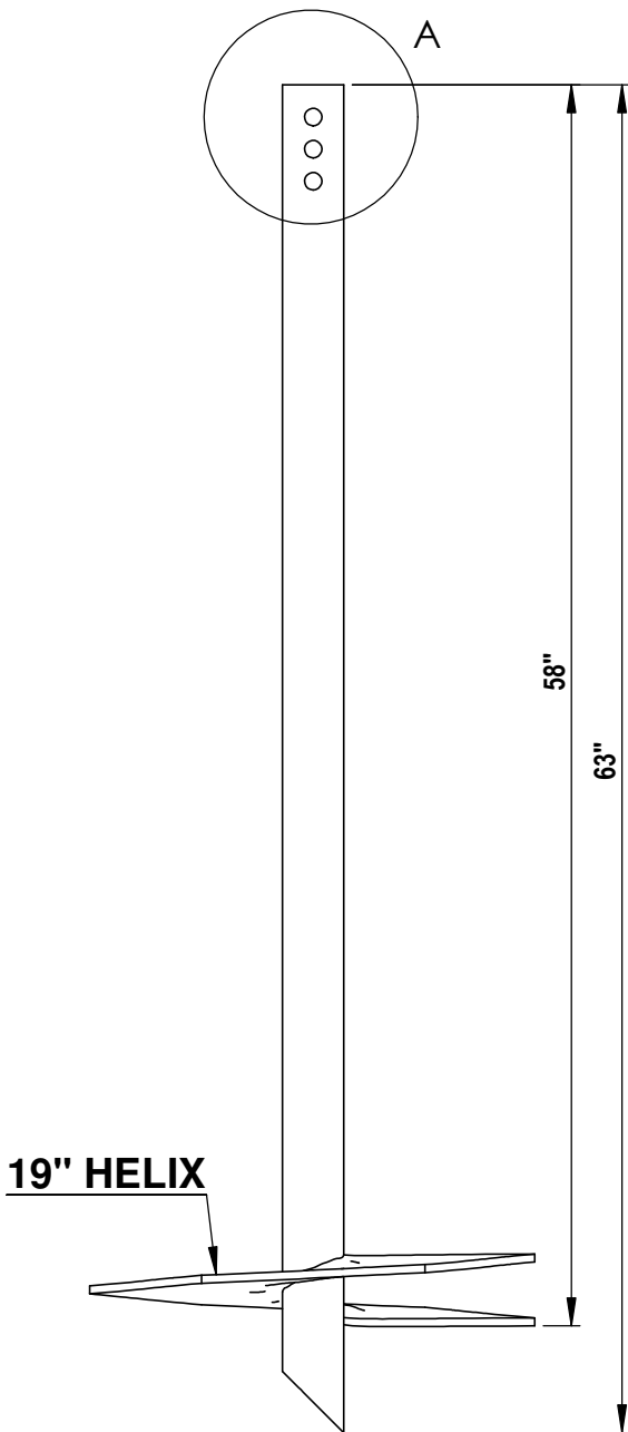
1 2.5" SCH40 SINGLE HELIX 1:10
